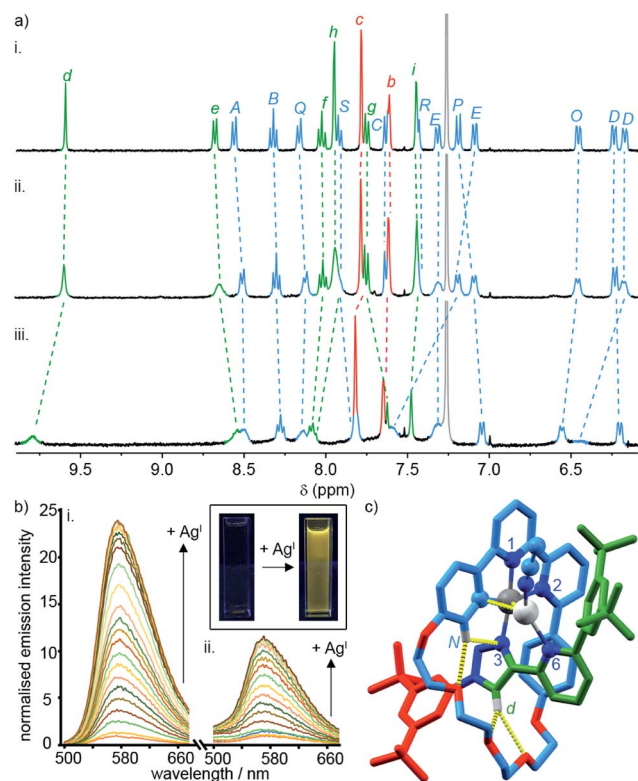
Fig. 4 (a) Partial 1 H NMR of (i) [Pt(κ 4 -4)]BF 4 , (ii) [Pt(κ 4 -4)]BF 4 + 1 equiv. AgSbF 6 , (iii) [Pt(κ 4 -4)]BF 4 + 1 equiv. of [Cu(MeCN) 4 ]PF 6 . (b) Photoluminescence response of (i) [Pt(κ 4 -4)]BF 4 and (ii) [Pt(2)(5)]BF 4 to the portion-wise addition of AgSbF 6 (inset: visual demonstration of the luminescent switch-on of [Pt(κ 4 -4)]BF 4 in the presence of 10 equiv. of Ag + ). (c) Solid-state structure of [Pt(κ 4 -4)Ag(MeCN)]BF 4 in partial sticks (rotaxane framework)/ball-and-stick (metals and ligand sphere) representation (anions and majority of Hs omitted for clarity). Colours: H white, C as in Scheme 2, N dark blue, O red, Pt dark grey, Ag light grey. Selected distances (Å) and angles (°): Pt–C 1.98, Pt–N1 1.95, Pt–N2 2.17, Pt–N3 2.02, Ag–Pt 2.83, Ag–C 2.54, H d –O 2.28, H d –O 2.60, H N –N3 2.51, H N –O 2.59, C–Pt–N2 161.3, N1–Pt–N3 172.1, C–Pt–N1 82.2, N1–Pt–N2 79.1, N2–Pt–N3 108.4, N3–Pt–C 90.3.
