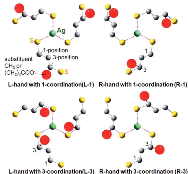
Fig. 4 Four possible combinations between the handedness of the NC and ( R )-ligand coordination orientation represented by the face-capping Ag-centered coordination unit (Ag(dithiolate) 3 unit) as a part of the NC structure.
