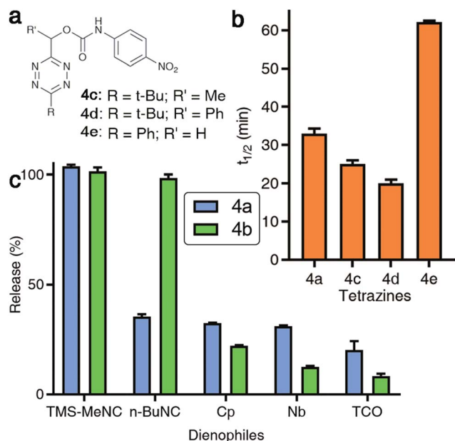
Fig. 3 Effect of structural modifications to tetrazines on isonitrile-induced removal. (a) Structures of modified Tzme probes with a pNA reporter molecule. (b) Half-lives of the TMS-MeNC mediated Tzme deprotection ( t_{1/2} of release of pNA) from probes 4a , 4c , 4d , and 4e ( c(\mathbf{4a-e}) = 0.2 mM, c(\text{TMS-MeNC}) = 2 mM, DMSO : PBS pH 7.4 (4 : 1, v/v), T = 37 °C). (c) Release yields of pNA or O-carboxymethyl fluorescein from 4a or 4b , respectively, triggered by several dienophiles (structures shown in Fig. S10 in the ESI†); pNA release: see Fig. 2d; t = 8 h; O-carboxymethyl fluorescein release: c(\mathbf{4b}) = 8 \mu M, c(\text{dienophile}) = 2 mM, DMSO : PBS pH 7.4 (1 : 4, v/v), T = 37 °C, \lambda_{\text{ex}} = 488 nm, \lambda_{\text{em}} = 520 nm, t = 8 h.
