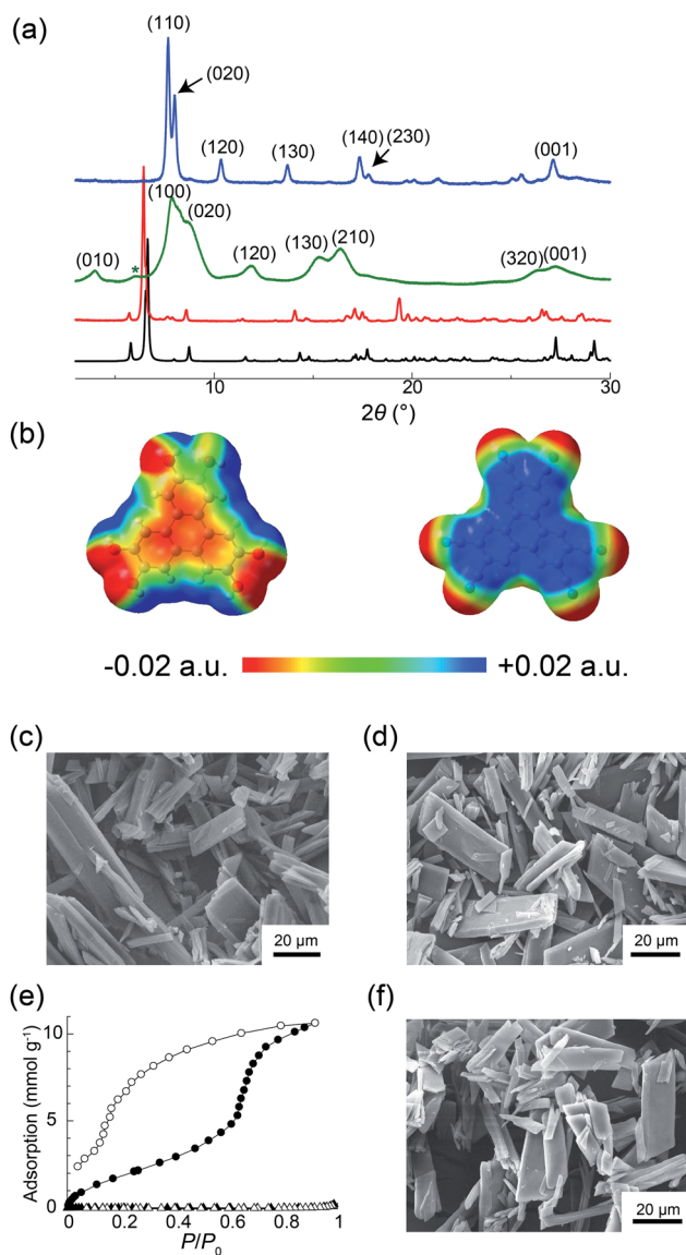
Fig. 3 (a) Simulated XRPD pattern of PCT-1 ·DMF (black) and experimental XRPD patterns of PCT-1 ·DMF (red), PCT-1 (green), and PCT-1 ·H 2 O (blue). The green asterisk indicates the background signal from the Kapton film that shields the sample from ambient air. (b) Electrostatic potentials (ESPs) of HHTP (left) and HAT-CN (right) in the crystal structure of PCT-1 ·DMF. SEM images of (c) PCT-1 ·DMF and (d) PCT-1 . (e) Adsorption (open symbols) and desorption (solid symbols) isotherms for H 2 O at 298 K (circles) and N 2 at 77 K (triangles). (f) SEM image of PCT-1 after water adsorption.
