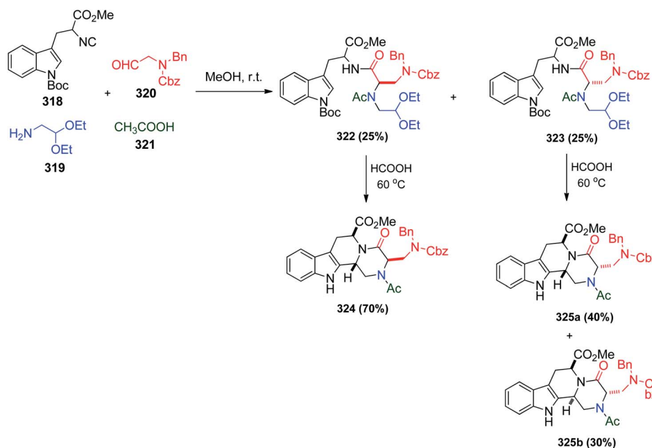
Scheme 68 Synthesis of 1,2,3,4-tetrahydro- \beta -carboline 324 and 325a and b via U-4CR/Pictet-Spengler reaction.
