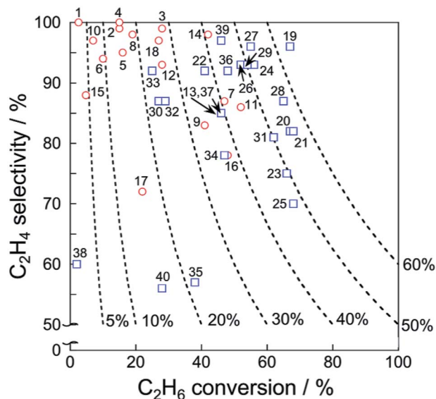
Fig. 11 Ethylene selectivity vs. ethane conversion of each catalyst presented in Tables 1 and 2. Dashed lines represent ethylene yield. Also, EDH in the absence and presence of \text{CO}_2 are shown respectively with red circles and blue squares.
