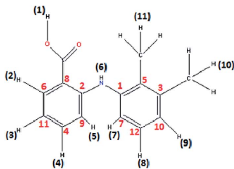
Fig. 1 Mefenamic acid (Hmef) with H and C atom numbering in accordance to ^1\text{H} NMR proton's assignment and ^{13}\text{C} NMR carbon's assignment.
