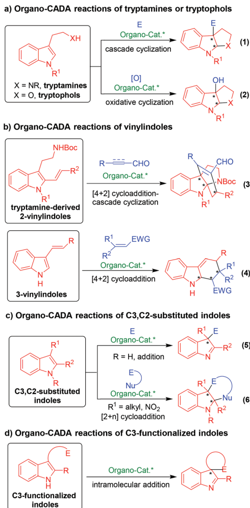
Scheme 1 Organo-CADA reactions of indole derivatives.
