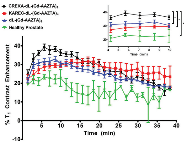
Fig. 5 In vivo MRI results from a multimeric AAZTA targeted CA (Fig. 4c) in PC3 orthotopic tumour bearing mice. Left: 7 T MRI images of prostate cancer in the mouse. (A) T_2 -Weighted image for tumour localisation; (B) T_1 -weighted image pre-injection of the CA; (C) T_1 -weighted image of the tumour region at 12 min post injection. Right: T_1 contrast enhancement (%) over time of the targeted CA (black), non-targeting scrambled peptide derivative (red) and non-functionalised variant (blue) in PC3 prostate cancer bearing mice. The green line represents the T_1 contrast enhancement of the targeted CA in healthy mice. Adapted with permission from ref. 99. Copyright © 2018 International Society for Magnetic Resonance in Medicine.
