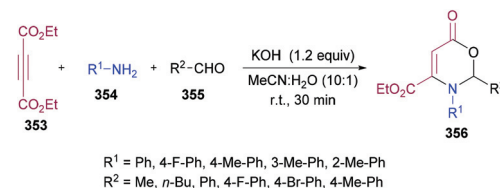
Scheme 90 Three-component synthesis of polysubstituted 2,5-dihydro-1,3-oxazin-6-ones from alkynoates, amines and aldehydes.
