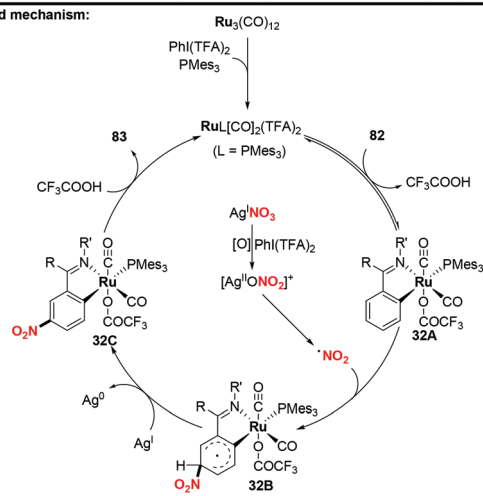
Scheme 32 Ruthenium-catalyzed PMes 3 -promoted meta -C-H nitration of arenes.
