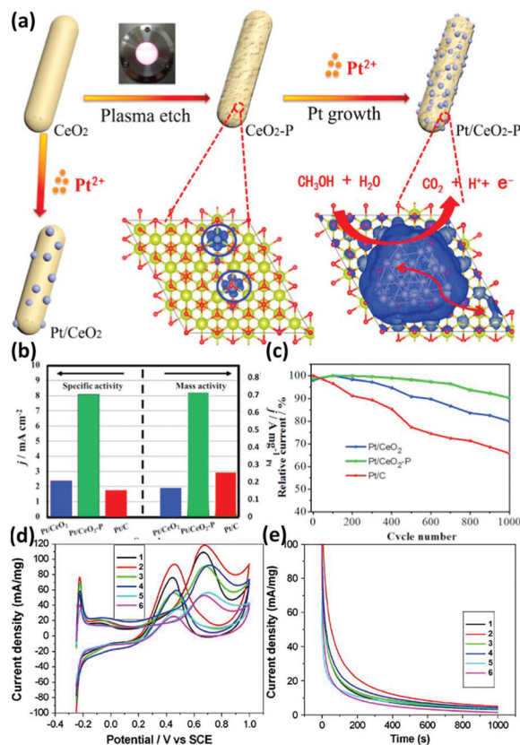
Fig. 21 (a) Schematic illustration of the mechanism of the Pt/CeO2 catalyst for the MOR. (b) Mass activity and specific activity for the MOR. (c) Stability test for the MOR. Adapted with permission from ref. 131. Copyright 2018, Elsevier. (d) Cyclic voltammograms and (e) chronoamperometry curves at 0.65 V (vs. SCE) for Pt/C and Pt/RE-C catalysts: Sample 1, Pt/Pr3Ce1O2-C; Sample 2, Pt/Pr1Ce1O2-C; Sample 3, Pt/Pr1Ce3O2-C; Sample 4, Pt3/PrOx-C; Sample 5, Pt3/CeOx-C; and Sample 6, Pt/C. Adapted with permission from ref. 133. Copyright 2008, Elsevier.
