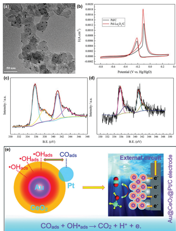
Fig. 20 (a) TEM image of Pd-L2O3/C. (b) Cyclic voltammograms of Pd/C and Pd-L2O3/C in 1 M KOH + 1 M CH3OH. XPS spectra of Pd 3d for (c) Pd/C and (d) Pd-L2O3/C. Adapted with permission from ref. 129 Copyright 2019, Elsevier. (e) Schematic illustration of the possible mechanism of Au@CeO2@Pt/C for the MOR. Adapted with permission from ref. 130. Copyright 2019, Royal Society of Chemistry.
