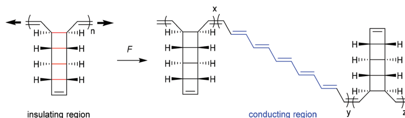
Scheme 13 Mechanical unzipping of poly ladderrenes.
