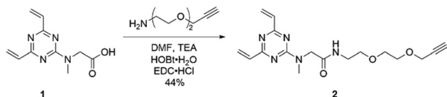
Scheme 1 Amide coupling of PEG 2 -alkyne unit to form triazine 2 .
