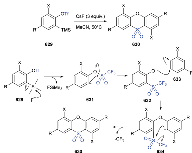
Scheme 95 Formation of phenoxathiine-dioxide derivatives via tandem anionic thia-Fries rearrangement-cyclisation of 2-(trimethylsilyl)phenyl trifluoromethanesulfonate benzyne precursors.
