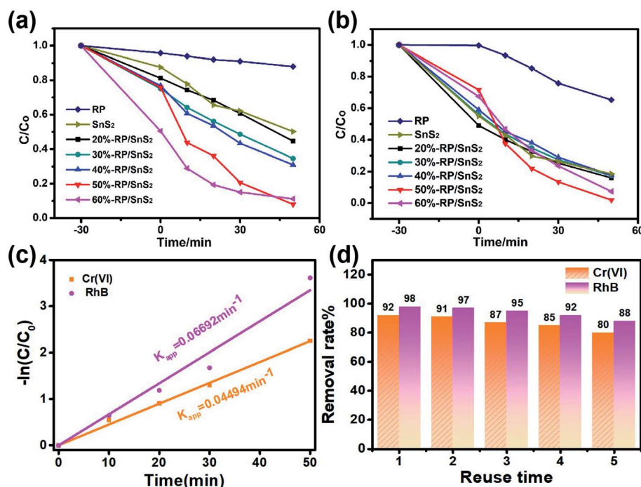
Fig. 2 Comparison of the effect of photocatalytic simultaneous removal of (a) \text{Cr}(\text{VI}) and (b) RhB by RP, \text{SnS}_2 , and x-RP/ \text{SnS}_2 . (c) the fitted reaction kinetic curves ( -\ln(C/C_0) = kt ) and (d) recycling test runs for five times in the photocatalytic removal of \text{Cr}(\text{VI}) and RhB by 50%-RP/ \text{SnS}_2 .
