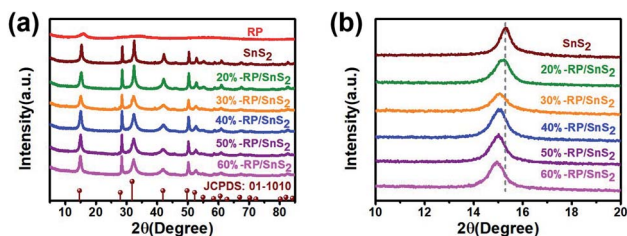
Fig. 1 XRD patterns of (a) full spectra and (b) magnified spectra of samples RP, \text{SnS}_2 , and x-RP/ \text{SnS}_2 .
