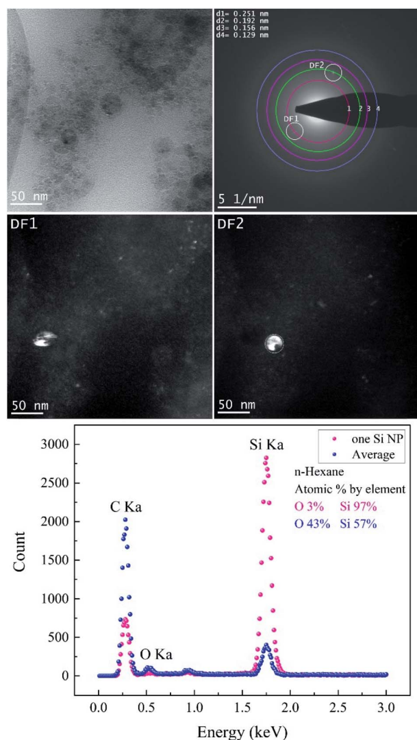
Fig. 7 The femtosecond laser-synthesized Si nanoparticles in n -hexane. ( N = 1000 , F = 10.46 \text{ J cm}^{-2} ). The TEM bright-field image, SAED pattern (upper right) and dark-field images related to different diffracted electron beams along the 1 st and 2 nd ring. The EDX spectrum from several small Si NPs and one Si NP.
