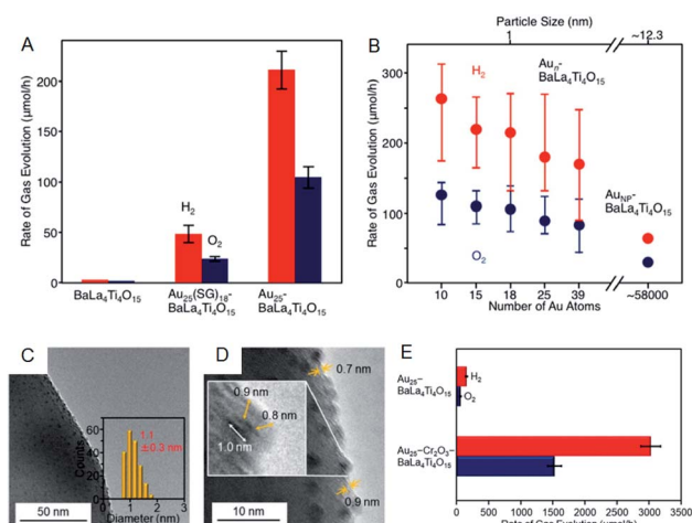
Fig. 10 Effect of (A) ligands protection and (B) cluster size on the rates of photocatalytic activity for water splitting studied using Au n /BaLa 4 Ti 4 O 15 ( n = 10\text{--}39 ) and Au NPs/BaLa 4 Ti 4 O 15 . (C) TEM image. (D) High resolution-TEM image. (E) Rates of photocatalytic activity for water splitting of Au 25 -Cr 2 O 3 /BaLa 4 Ti 4 O 15 . Panels (a) and (b) are reproduced with permission from ref. 60. Copyright 2015 American Chemical Society. Panels (c)–(e) are reproduced with permission from ref. 61. Copyright 2018 American Chemical Society.
