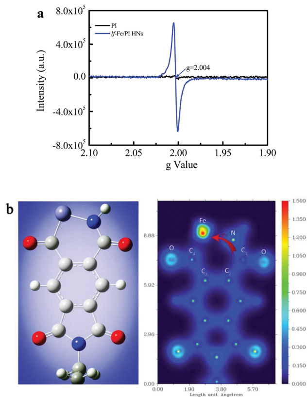
Fig. 4 Non-uniform distribution of surface electrons on lf-Fe/PI HNs. (a) EPR spectra of PI and lf-Fe/PI HNs. (b) DFT calculations for the optimized structure of lf-Fe/PI HNs in one unit (left) and the corresponding two-dimensional valence-electron density color-filled maps of the lf-Fe/PI HNs model (right). Purple, red, grey and blue circles denote Fe, O, C and N atoms, respectively. The valence-electron density is given in \text{e} \text{Å}^{-3} .
