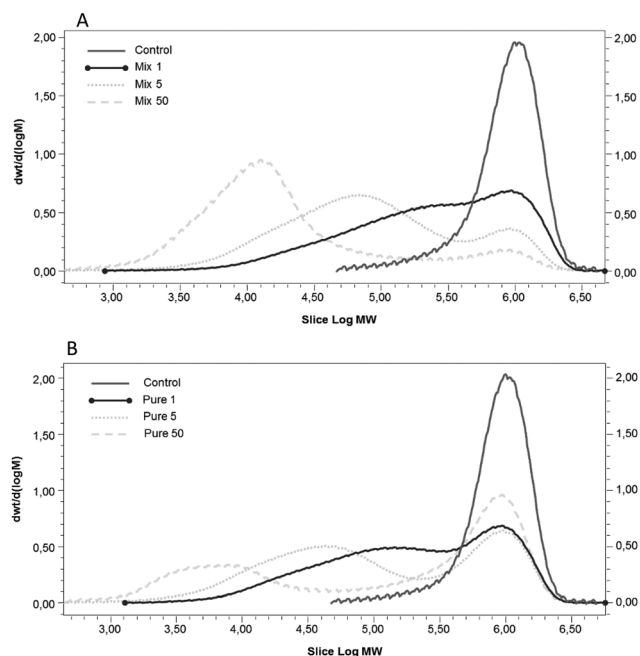
Fig. 2 Molecular weight distribution of \beta -glucan in OBC enzymatically treated with (A) Mix and (B) Pure enzymes (1, 5 or 50 nkat g^{-1} ). Control refers to the OBC treated under the same conditions but without any enzyme.
