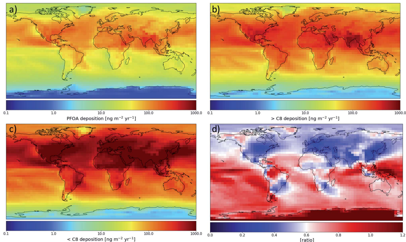
Fig. 2 Spatial distribution of modeled 2013–2015 annual average (a) PFOA deposition ( \text{ng per m}^2 \text{ per year} ), (b) deposition of all longer-chain PFCAs ( \text{ng per m}^2 \text{ per year} ), (c) deposition of all shorter-chain PFCAs, and (d) precursor-produced long-chain (>C7) to short-chain deposition ratio.
