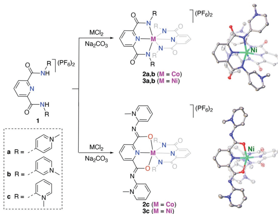
Scheme 1 Synthesis of Co(II) and Ni(II) bis-pyPYA 2 pincer complexes 2a–c and 3a–c in H 2 O/EtOH (1:1 v/v). Crystal structures of complex cations 3b and 3c ; all ellipsoids at 50% probability level (hydrogen atoms and co-crystallized solvent molecules omitted for clarity).
