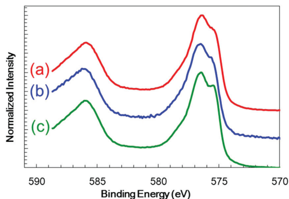
Fig. 2 XPS spectra obtained from a \text{Cr}_2\text{O}_3 electrode (a) before and (b) after photoelectrolysis for 1 h and from (c) the reference \text{Cr}_2\text{O}_3 .
