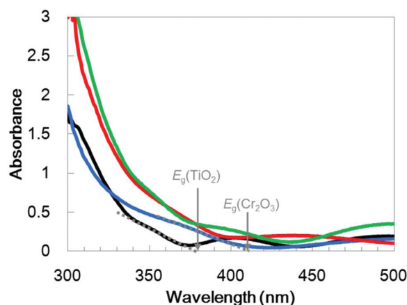
Fig. 4 UV/visible absorption spectra for \text{TiO}_2/\text{Cr}_2\text{O}_3 (red line), \text{Cr}_2\text{O}_3 (blue line) and \text{TiO}_2 (black line) on TCO and the sum of the \text{Cr}_2\text{O}_3 and \text{TiO}_2 spectra (green line). E_g indicates the absorption edges for the band-gap excitation.
