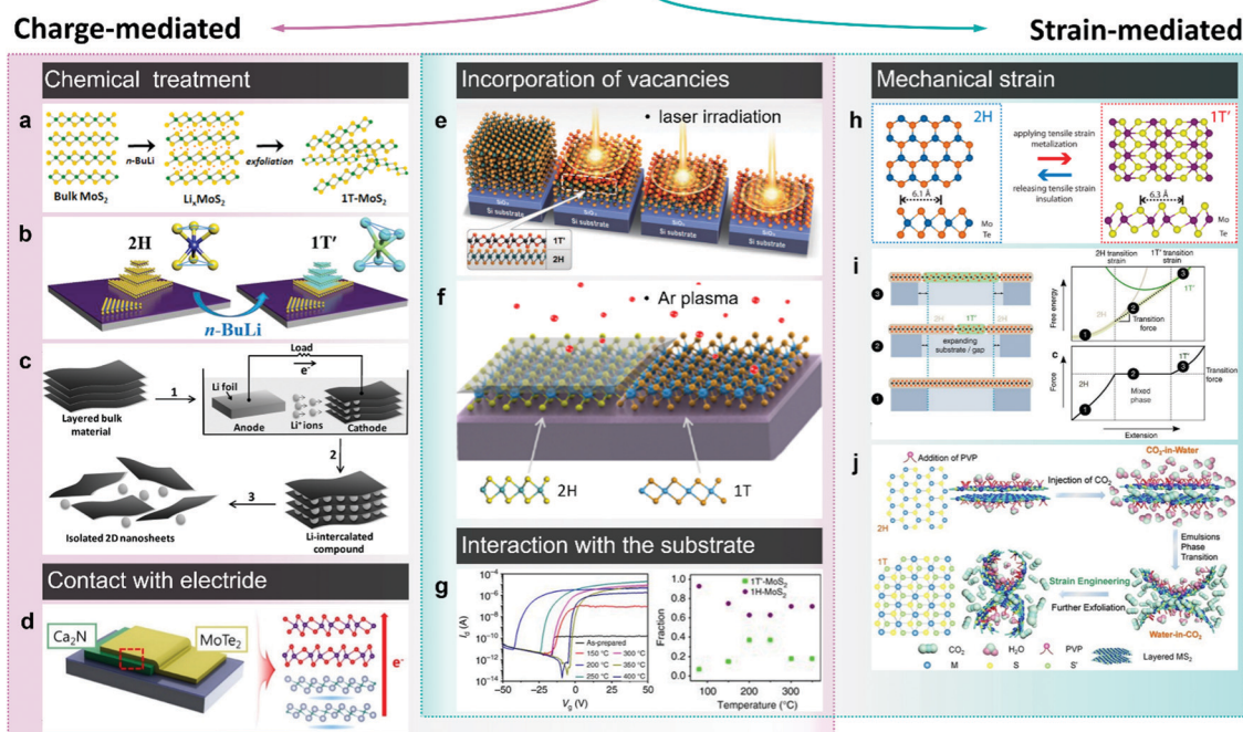
Fig. 3 Accessing the metastable 1T(1T') phase via destabilisation of the thermodynamically stable (2H) phase. The approaches to induce the 2H-to-1T' transition in group VI TMDs are divided in two categories: charge-mediated, as chemical treatment (panels a–c) and contact with an electrode (panel d); and strain-mediated, such as tensile strain-induced transition between the 2H and 1T'(1T) polymorphs (panels h–j). Panels e–g represent the phase transitions caused by the combination of charge and strain as in the case of chalcogen vacancies (panels e and f) or due to the interaction with the substrate (panel g). Separate panels are adapted with permission: (a) from ref. 100, copyright 2017, American Chemical Society; (b) from ref. 114, copyright 2018, American Chemical Society; (c) from ref. 108, copyright 2011, John Wiley & Sons; (d) from ref. 123, copyright 2017, American Chemical Society; (e) from ref. 155, copyright 2015, American Association for the Advancement of Science; (f) from ref. 138, copyright 2017, American Chemical Society; (g) from ref. 128, copyright 2017, Springer Nature; (h) from ref. 130, copyright 2016, American Chemical Society; (i) from ref. 25, copyright 2014, Springer Nature; and (j) from ref. 134, copyright 2017, John Wiley & Sons.
