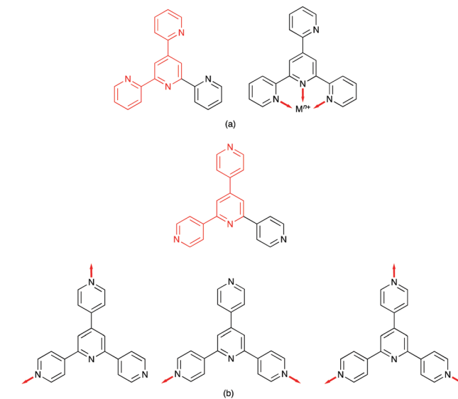
Scheme 2 Examples of tpty motifs as units within quaterpyridines. (a) 4'-(Pyridin-2-yl)-2,2':6',2''-tpty contains a 2,2':4',2''-tpty unit (in red) but typically binds metal ions as a bis(chelate). (b) 4'-(Pyridin-4-yl)-4,2':6',4''-tpty contains a 4,2':4',4''-tpty unit (in red); three possible ditopic modes of bonding of 4'-(pyridin-4-yl)-4,2':6',4''-tpty represented in the CSD by refcode entries AGUPUO (left), QOTREY (middle) and RIGPII (right).
