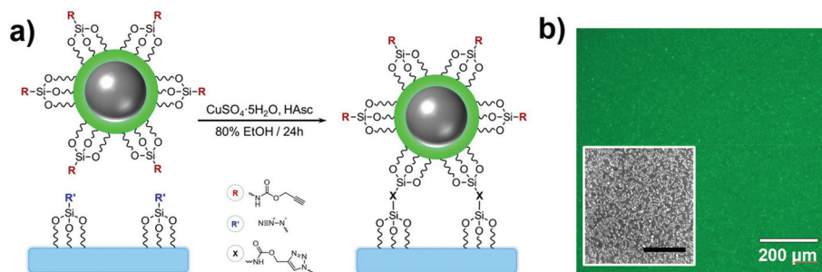
Fig. 10 (a) Grafting scheme of Ag@(FL) NPs to a SiO 2 substrate through Cu I -catalyzed 1,3-dipolar cycloaddition. (b) Fluorescence image of the substrate grafted with Ag@(FL) NPs ( \lambda_{exc} = 489 \pm 6 nm, \lambda_{em} = 536 \pm 20 nm). Inset: SEM image of a region the substrate (scale bar: 1 μm). Adapted from ref. 115 with permission from the Royal Society of Chemistry, Copyright 2014.
