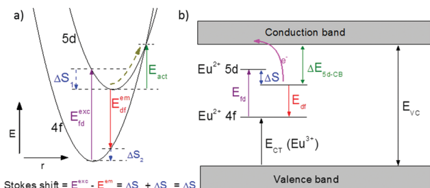
Fig. 1 (a) Configurational coordinate diagram of the 4f and 5d state of \text{Eu}^{2+} , with energy E versus configurational coordinate r , showing the mechanism of thermal quenching of the \text{Eu}^{2+} 5d–4f emission via the crossing point between the 5d and 4f parabola; (b) mechanism of thermal quenching of the \text{Eu}^{2+} 5d–4f emission by thermal ionization of the \text{Eu}^{2+} 5d electron to the host lattice conduction band, with energy difference \Delta E_{5d\text{-CB}} between the relaxed 5d state and the bottom of the conduction band.
