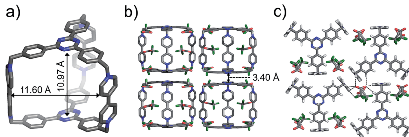
Fig. 2 Solid-state (super)structures of AzaEx 2 Cage ·6CF 3 CO 2 obtained by single-crystal X-ray crystallography. (a) Stick representation of AzaEx 2 Cage 6+ , CF 3 CO 2 − counterions are omitted for the sake of clarity. (b and c) Side-on views of the packing structure revealing that \pi – \pi and hydrogen-bonding interactions play important roles in the crystal packing. The close contacts in the range of 2.22–2.46 Å between CF 3 CO 2 − counteranions and the protons in the cage indicate the occurrence of Hydrogen-bonding interactions, which are labeled with dashed lines. Hydrogen atoms and disordered solvent molecules are omitted for the sake of clarity. C, gray; N, blue; F, green; O, red.
