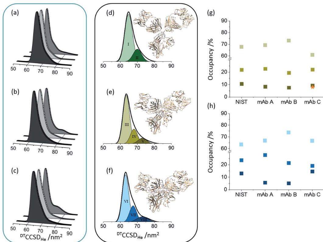
Fig. 2 Global collision cross section distributions ( ^{DT}CCSD_{H_{90}} ) for intact (a), endoS2 treated (b) and deglycosylated (c) Herceptin®; lot A (dark grey), lot B (light grey) and lot C (grey). Global CCSDs for intact (d), endoS2 treated (e) and deglycosylated (f) NIST mAb standard with fitted conformers. The darker the Gaussian for each sample, the more extended the conformer. The conformers present in each sample preparation have slightly different centres and FWHM values, hence different colours for each sample preparation. CCSDs for individual charge states for each sample and at each glycosylation level are provided in Fig. S7 in ESI.† Inserted mAb figures are snapshots from MD trajectories previously performed on pdb: 1IGY. 30 The image in (d) is from early in the MD simulation and therefore represents the intact mAb; later snapshots represent more contracted forms (e and f). Percentage occupancies of each conformer in the endoS2 treated samples (g) and deglycosylated samples (h) are presented with colours corresponding to the fitted Gaussians. For the endoS2 treated Herceptin® lot C there is an additional fourth extended Gaussian (see Fig. S6 in ESI†) which is represented by the orange star. Standard deviations between three day-to-day replicates are provided for the ^{DT}CCSD_{H_{90}} for individual charge states in Fig. S7 in ESI.†
