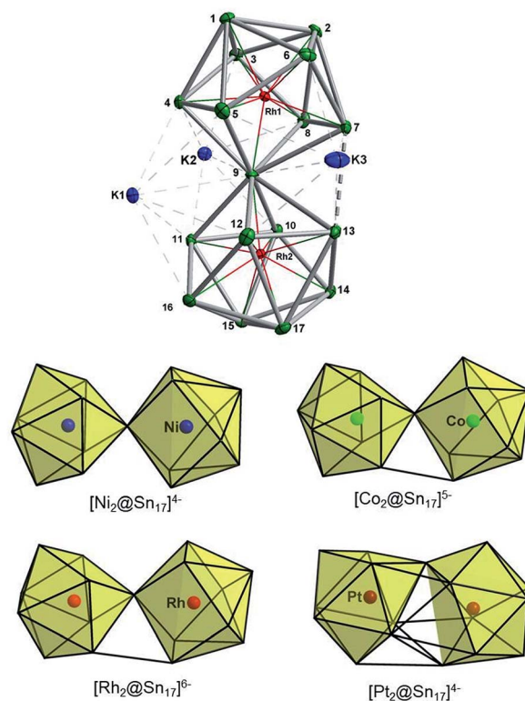
Fig. 4 Top: Thermal ellipsoid plots of the [\text{Rh}_2\text{Sn}_{17}]^{6-} anion and its three tightly bound K^+ cations (drawn at 50% probability). Bottom: Comparison of the known structures of M_2\text{Sn}_{17} anions, M = \text{Ni} , 18a \text{Co} , 5b \text{Rh} and \text{Pt} . 18b
