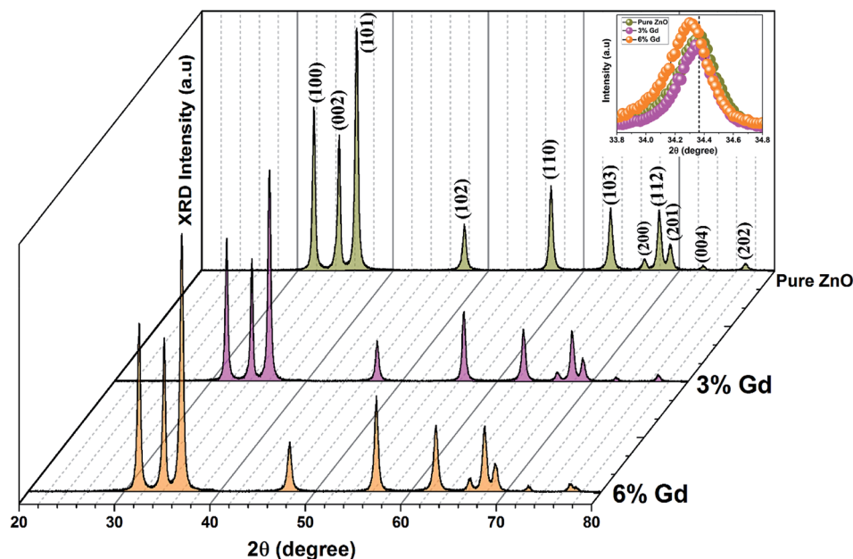
Fig. 1 X-ray diffraction patterns of pristine and Gd-doped ZnO-NRs annealed at 400 °C for 1 h. The X-ray diffractograms show that the prepared samples are polycrystalline with hexagonal wurtzite phase. The inset shows the shift of the diffraction peak along (002) plane at varying doping concentrations.
