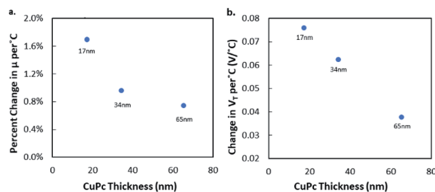
Fig. 4 Effect of CuPc thickness on BGBC OTFTs performance as a function of temperature (between 25 ^{\circ}\text{C} and 85 ^{\circ}\text{C} for air and 20 ^{\circ}\text{C} to 150 ^{\circ}\text{C} for vacuum). (a) % change in hole mobility, \mu_H compared to baseline at 25 ^{\circ}\text{C} per ^{\circ}\text{C} and (b) the change in threshold voltage V_T per ^{\circ}\text{C} .
