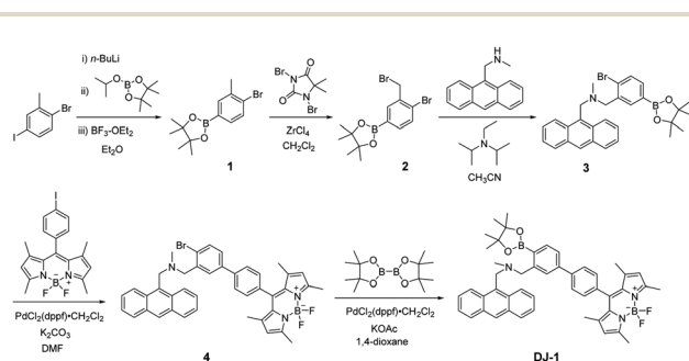
Scheme 1 Synthesis of DJ-1 .
