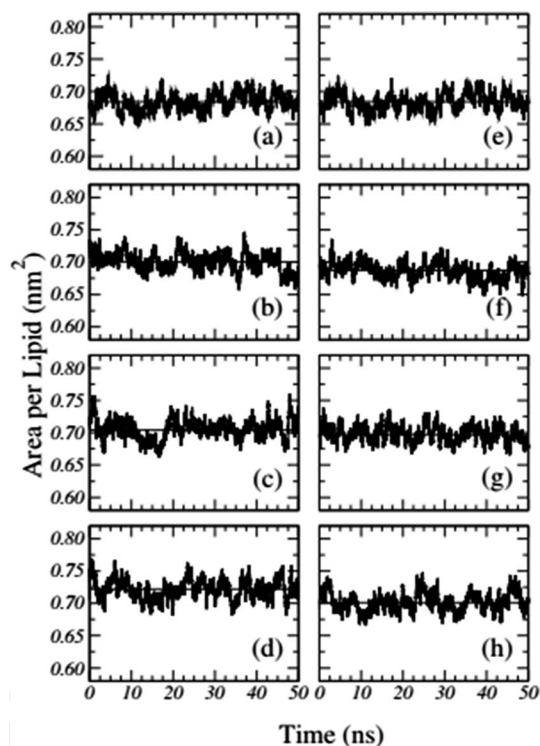
Fig. 1 Time-dependent area per lipid in the presence of GLYP2 (left column) and GLYP (right column) at different G : L ratios of (a) and (e) 0 : 72; (b) and (f) 1 : 18; (c) and (g) 1 : 9 and (d) and (h) 1 : 3. Horizontal solid lines represent the mean average value of the area per lipid for the last 40 ns of the simulation. Reproduced from ref. 68 with permission from Elsevier.
