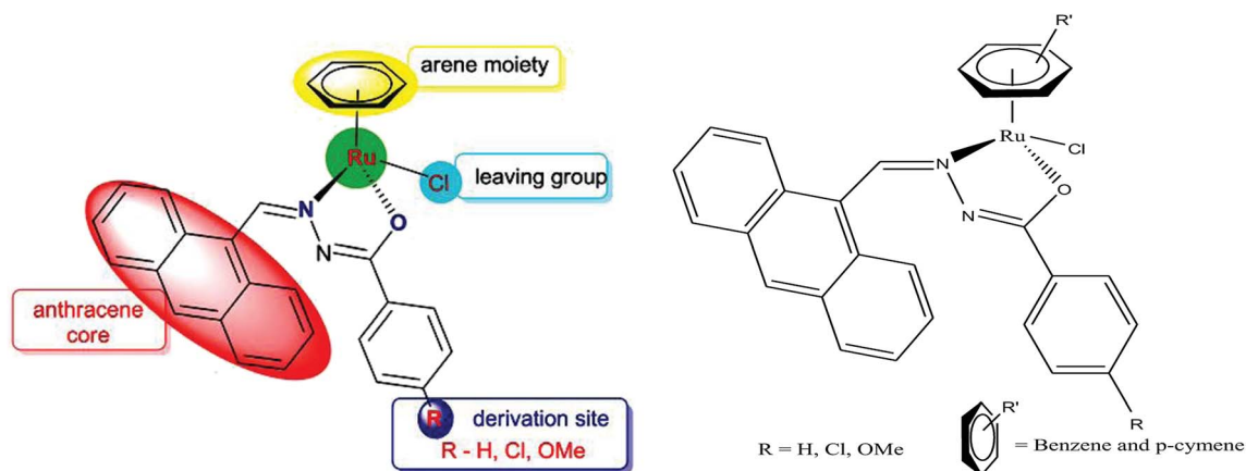
Fig. 6 Design of ligand framework and chemical structure of organometallic ruthenium(II) arene 9-anthraldehyde benzhydrazone complexes. This figure was reproduced from ref. 66 with permission from the Royal Society of Chemistry (Great Britain).
