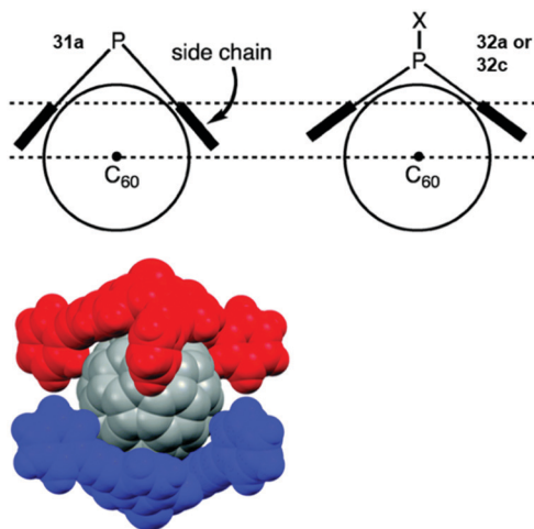
Fig. 43 Top: Illustration of the coordination of a P-centered triangulene with a deep ( 31a ) and a shallow bowl ( 32a/c ) to C_{60} . Bottom: Space-filling model of the (( P )- 31a ) 2 · C_{60} complex. 20 Figure reproduced with kind permission; © 2015 The Royal Chemical Society.
