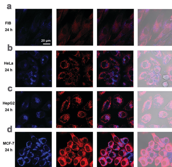
Fig. 3 Confocal laser scanning microscopy (CLSM) images of different cells stained by 0.1 mg mL -1 TCSC for 24 h, and then stained by MitoTracker ® Red CMXRos for TCSC NP localization. (a) FIB; (b) HeLa; (c) HepG2; (d) MCF-7. First column: TCSC particles (blue); second column: mitochondria (red); third column: merge images of two fluorescence channels; and fourth column: with corresponding bright field channel images, respectively.
