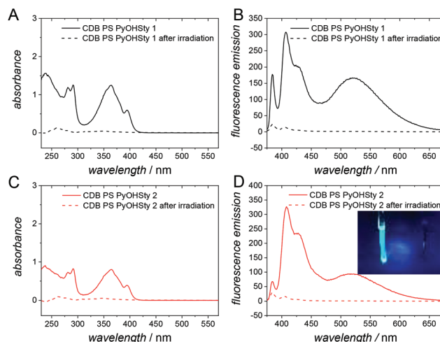
Fig. 4 UV Vis (A and C) and fluorescence spectra (B and D, \lambda_{exc.} = 344 \text{ nm} ) of CDB PS PyOHSty 1 and 2 before and after exposure to LED irradiation (430–435 nm) showing the presence of pyrene monomers and excimers before light-induced cleavage. The fluorescence of pyrene can also be detected via exposure of the NMR samples to a simple hand-held UV lamp ( \lambda_{exc.} = 366 \text{ nm} , part D, left: parent polymer, right: after LED light-induced cleavage).
