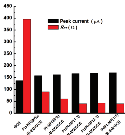
Fig. 3 Variation of the oxidation peak currents and R_{ct} of 5 mM [\text{Fe(CN)}_6]^{3-/4-} in 0.1 M KCl on a GCE, a Pd-NP(30%)/B-EG/GCE, a Pt NP(30%)/B-EG/GCE, a PdPt-NP(1:3)/B-EG/GCE, a PdPt-NP(3:1)/B-EG/GCE, and a PdPt-NP(1:1)/B-EG/GCE.
