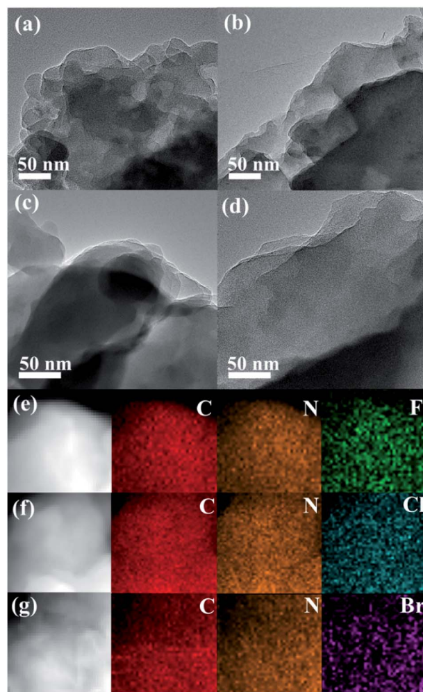
Fig. 1 TEM images of (a) CTF-1, (b) CTFF, (c) CTFCl and (d) CTFBr. EDX elemental mappings of (e) CTFF, (f) CTFCl and (g) CTFBr.
