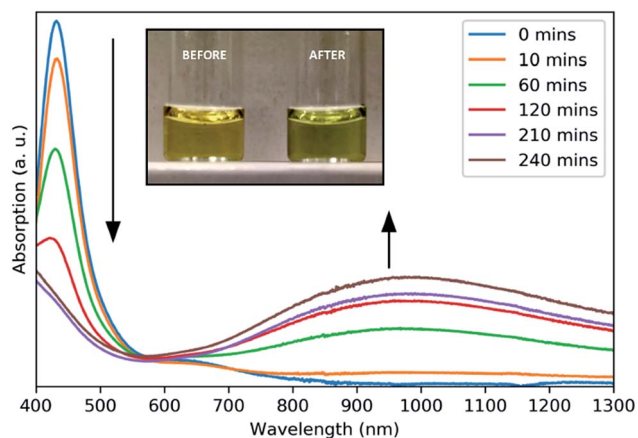
Fig. 2 Absorbance spectra of aliquots taken at intervals throughout the growth of CuS NCs. Inset: a photograph of the reaction solution before and after heating.
