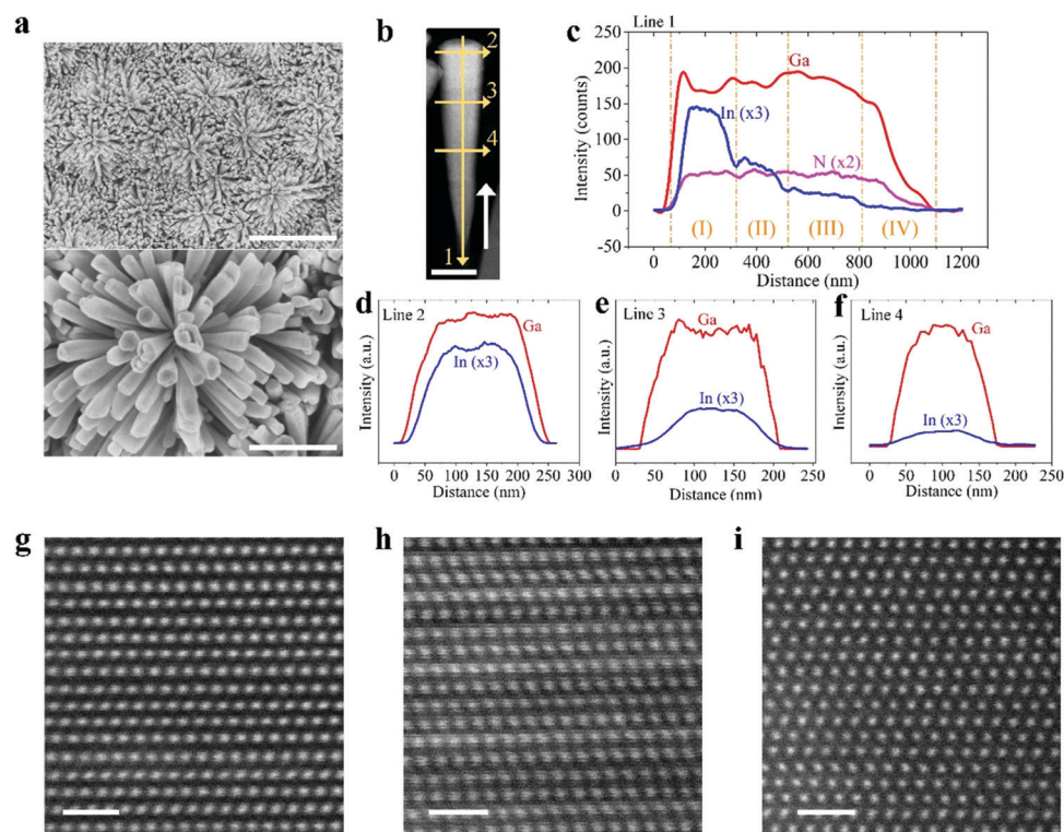
Fig. 3 Structural characterization of the quadruple-band InGa N nanowire arrays monolithically integrated on a nonplanar Si wafer. (a) Top-view scanning electron microscopy (SEM) images of the flower-shaped InGa N nanowire structure grown on nonplanar Si substrates. Scale bar: 5\ \mu\text{m} (top) and 1\ \mu\text{m} (bottom). (b) Dark-field scanning transmission electron microscopy (DF-STEM) image of the quadruple-band InGa N nanowire, with energy-dispersive X-ray spectroscopy (EDX) line scanning showing the variation of Ga L \alpha , In L \alpha , and N K \alpha characteristic signals along the axial and lateral directions. Scale bar: 200\ \text{nm} . Spectra of Line 1 (c), Line 2 (d), Line 3 (e), and Line 4 (f) are measured along Arrow 1, Arrow 2, Arrow 3, and Arrow 4 in (b), respectively. (g–i) Atomic resolution STEM images of InGa N crystals for (g) In 0.35 Ga 0.65 N, (h) In 0.27 Ga 0.73 N, and (i) In 0.20 Ga 0.80 N segments, respectively. Scale bar: 1\ \text{nm} .
