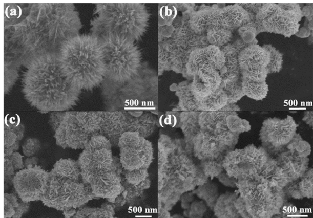
Fig. 4 SEM images of (a) bare \text{WO}_{2.72} , (b) pure \text{WO}_3 ( \text{WO}_{2.72} calcined at 450 °C for 1.5 h), (c) 0.25 mol% Fe-doped \text{WO}_3 (0.25 mol% Fe-doped \text{WO}_{2.72} calcined at 450 °C for 1.5 h), (d) 0.75 wt% Pt@0.25 mol% Fe- \text{WO}_3 after 9 time photocatalytic degradation experiments.
