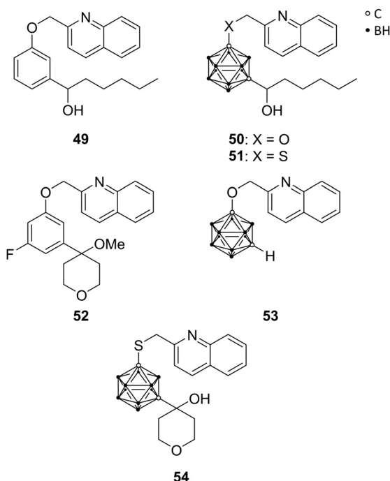
Fig. 14 Structures of 5-lipoxygenase inhibitors Rev-5901 49 , CarbORev-5901 50 , CarbSRev-5901 51 , ZD-2138 52 , meta -carborane analogue of 2-(phenoxy)methylquinoline 53 and the 4-hydroxytetrahydropyranyl carborane derivative 54 .
