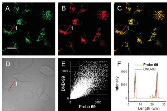
Fig. 117 Colocalization of 69 and DND-99 in A549 cells. Cells were grown under the hypoxic condition of 1\% \text{ O}_2 and then co-stained with 69 ( 2 \mu\text{M} ) and DND-99 ( 100 \text{ nM} ) at 37^\circ\text{C} . (A) Fluorescence image from the 69 channel ( \lambda_{\text{ex}} = 405 \text{ nm} , \lambda_{\text{em}} = 455\text{--}555 \text{ nm} ). (B) Fluorescence image from the DND-99 channel ( \lambda_{\text{ex}} = 559 \text{ nm} , \lambda_{\text{em}} = 570\text{--}670 \text{ nm} ). (C) Merged image of images (A) and (B). (D) Corresponding differential interference contrast (DIC) image. (E) Intensity correlation plot of 69 and DND-99. (F) Intensity profiles of 69 and DND-99 within the linear ROI 1 (red lines in A and B) across the cell. Scale bar, 20 \mu\text{m} . Copyright 2016 Wiley-VCH.
