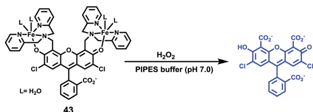
Scheme 32 Fluorescent probe 43 for H_2O_2 .
