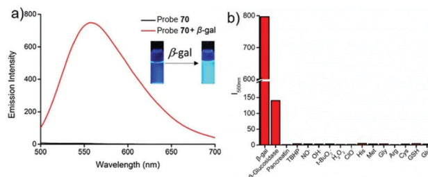
Fig. 118 (a) The emission of probe 70 with or without \beta -gal ( \lambda_{\text{ex}} = 460 \text{ nm} ). Inset: Images irradiated with 365 \text{ nm} ultraviolet light. (b) Fluorescence intensity of 70 ( 10 \mu\text{M} ) in response to the test species in a PBS buffer solution at 560 \text{ nm} excited at 460 \text{ nm} . Copyright 2017 Elsevier.
