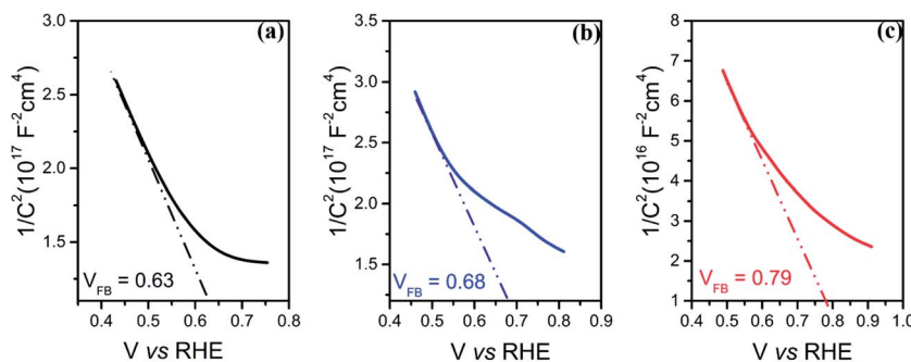
Fig. 6 Mott–Schottky measurements of (a) p-Si/TiO 2 (b) p-Si/TiO 2 /CoO x and (c) p-Si/TiO 2 /NiO x .
