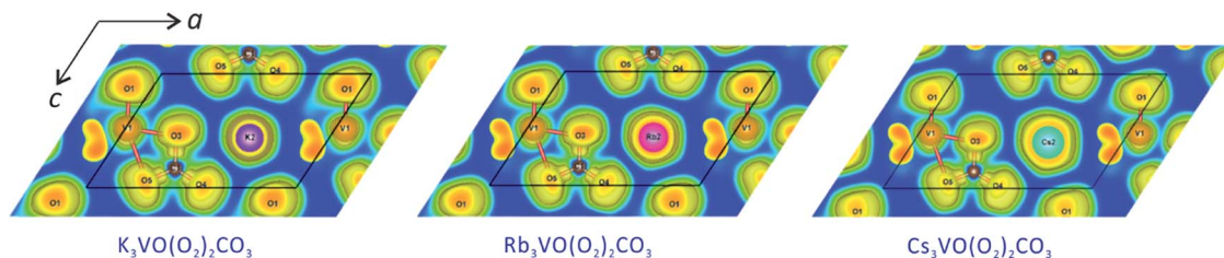
Fig. 5 Three sliced-planes of electron localization function (ELF) of A_3VO(O_2)_2CO_3 ( A = K, Rb , and Cs ) in the crystallographic ac -plane. All diagrams are depicted as filled contour maps. The color scheme ranges from blue to red ( 0-0.7 e^- per \text{\AA}^3 ), and values higher than 0.5 represent the area exceeding the free-electron ELF value. The unit cell is outlined in black.
