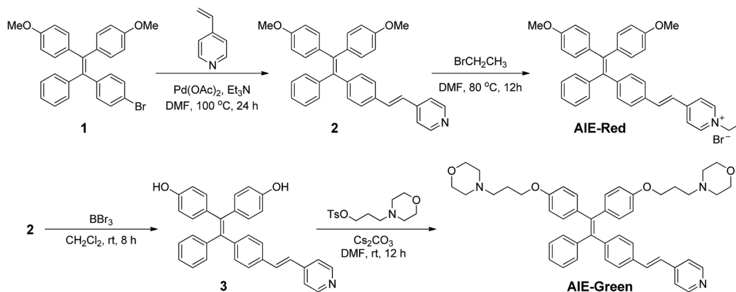
Scheme 2 The synthetic routes to obtain AIE-Red and AIE-Green (DMF represents dimethyl formamide).
