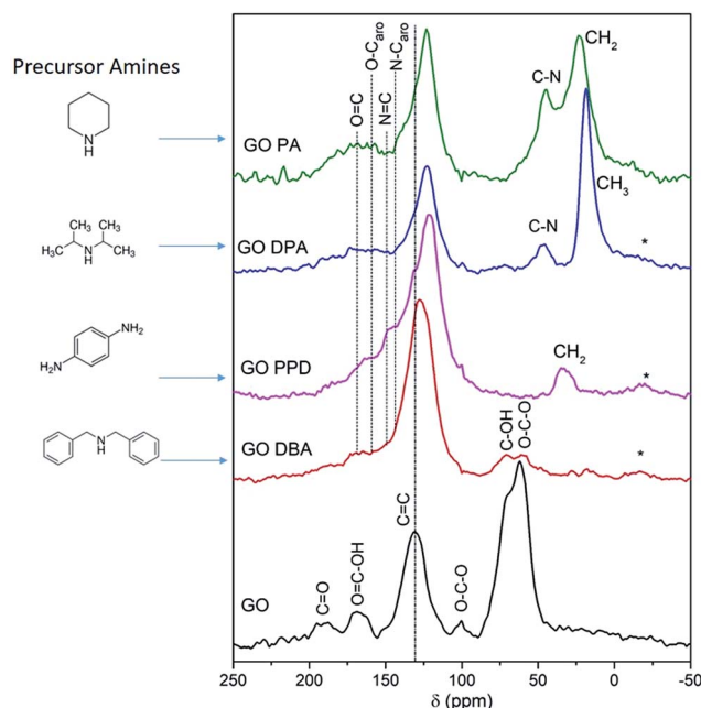
Fig. 7 13 C NMR spectra of GO and GO-amine. The asterisks indicate spinning sidebands.
