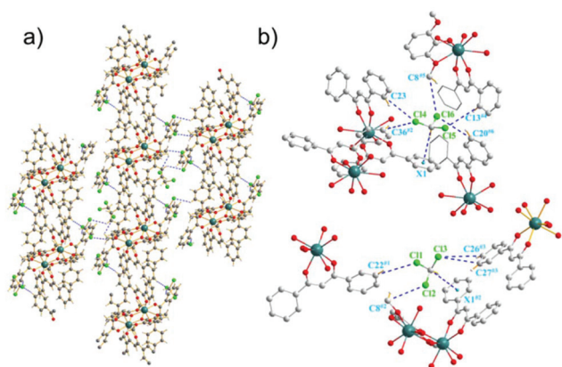
Fig. 2 (a) Crystal packing of 1 along the a -axis. Dy, dark blue; O, red; C, grey; H, white; Cl, green. (b) Views showing the C–H... \pi interactions and intermolecular H–C...Cl interactions among the crystallographically equivalent Dy–DMOP units of 1 (hydrogen atoms have been omitted for clarity; symmetry codes: #1: 1 - x, 1 - y, z ; #2: 1 - x, 1 - y, 1 - z ; #3: x - 1, y, z ; #4: 1 - x, -y, -z ; #5: x, y, z - 1 ; #6: 1 + x, y, z ).
